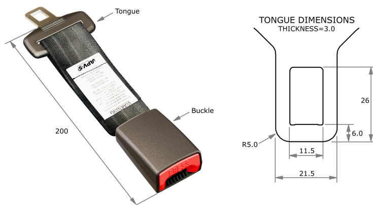
K6629 Extension Belt
