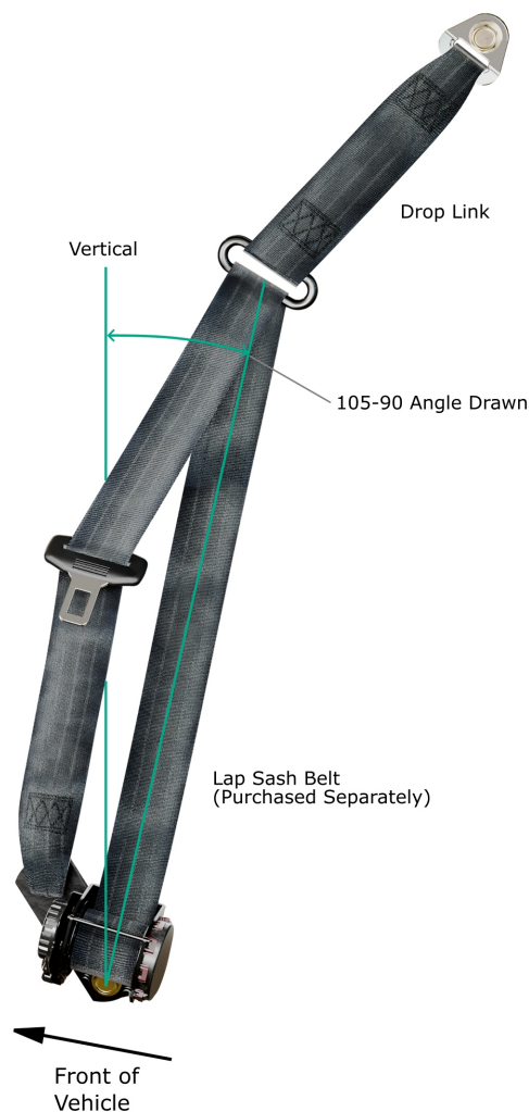
DROP LINK EXAMPLE
